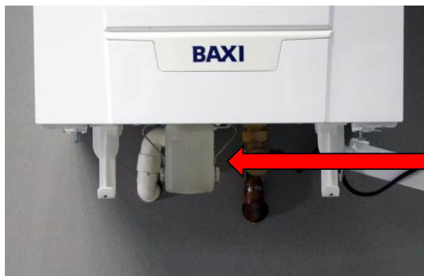
Figure 3 General Access - Location of condensate trap and retaining clip
